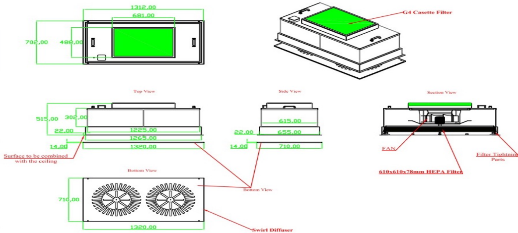
610x1220x78 Fan Filter Unit Filter Changing from Bottom
